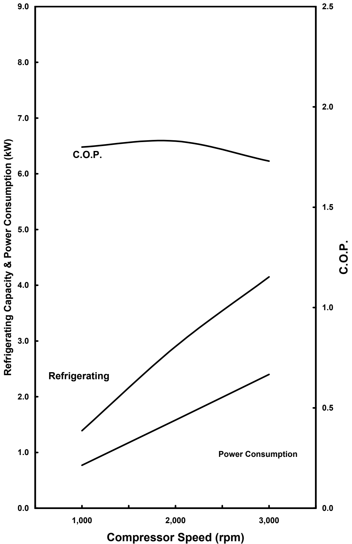
SD5H09 Performance
