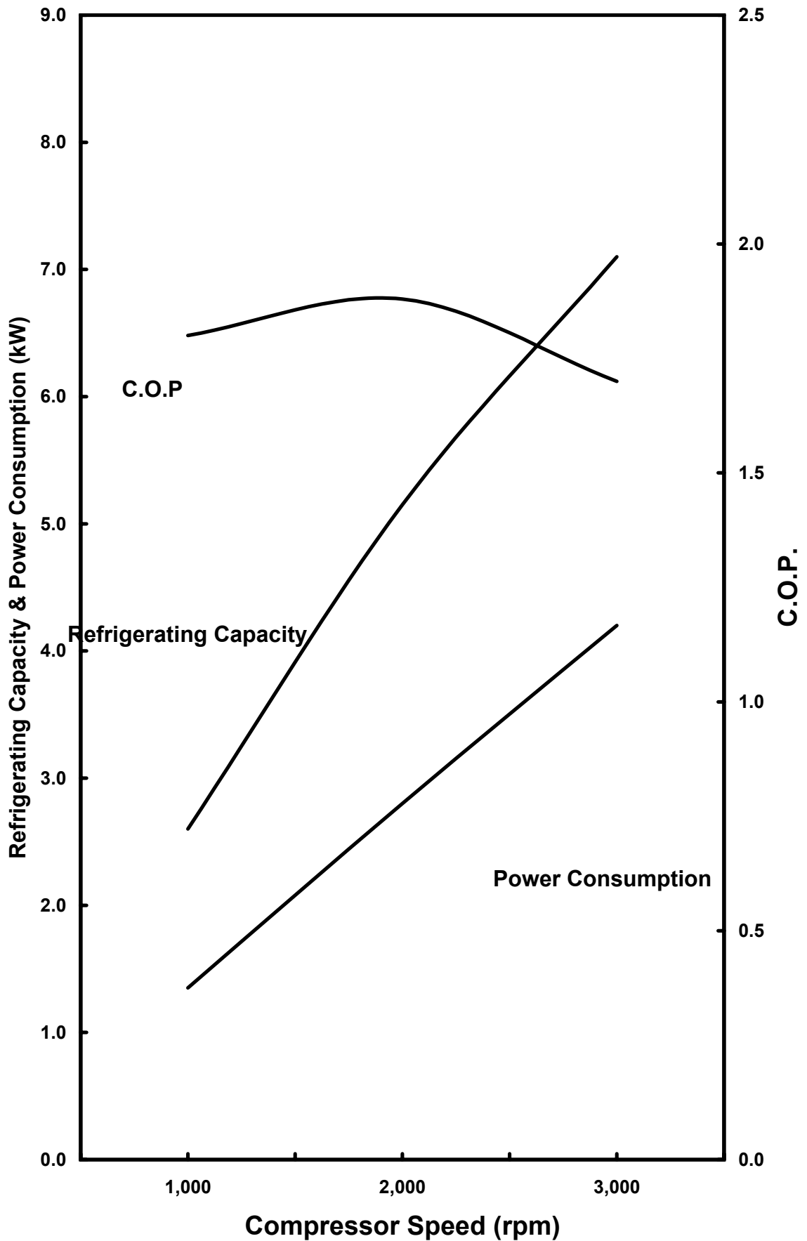
SD5H14 Performance
